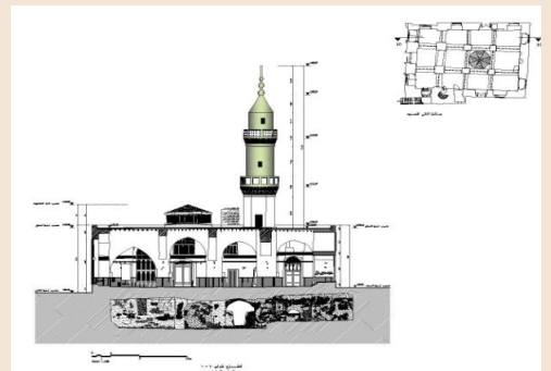
Longitudinal section before restoration
