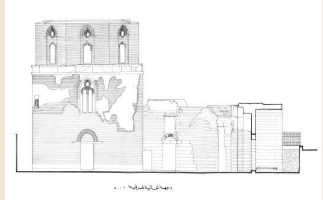
Fatma Khatun -Section ( CIAH)
