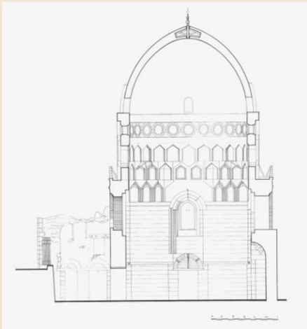
Ashraf Khalil Mausoleum- Section A-A (CIAH)
