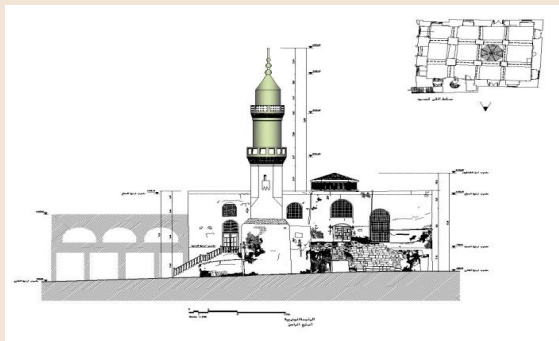
South Façade before restoration
